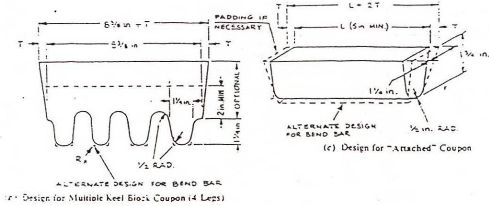
FIG. 16 Test Coupons for Castings (see Table 1 for Details of Design)
