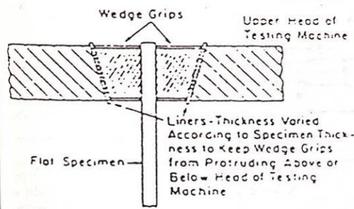
FIG. 2 Wedge Grips with Liners for Flat Specimens
