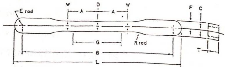
Dimensions, mm
