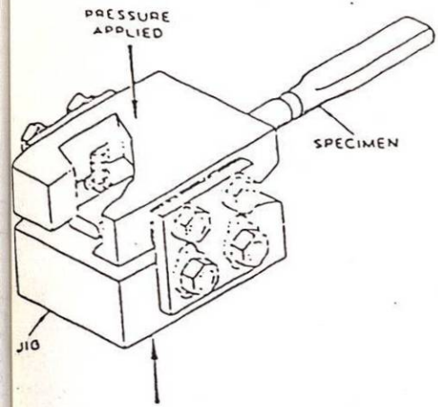
Squeezing Jig for Flattening Ends of Full-Size Tension Test Specimens
