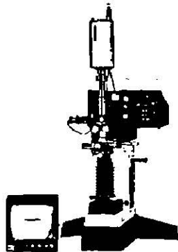
Microhardness Testers (shown here with video display)
