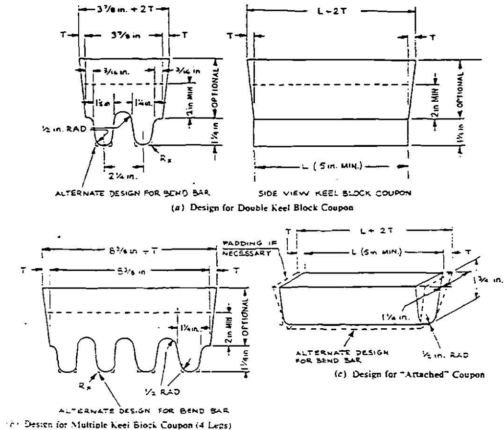
FIG. 16 Test Coupons for Castings (see Table 1 for Details of Design)
