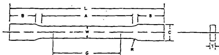
Dimensions, mm
