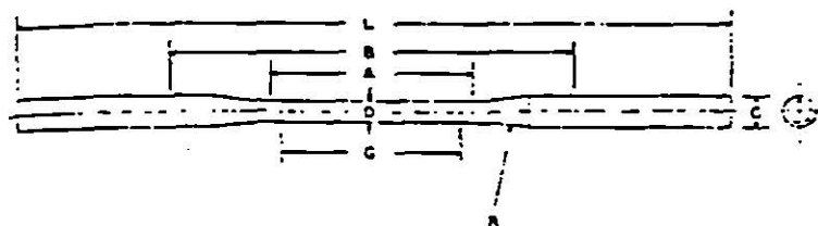
Dimensions, mm
