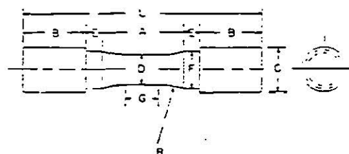
FIG. 13 Tension Test Specimens for Large-Diameter Tubular Products
