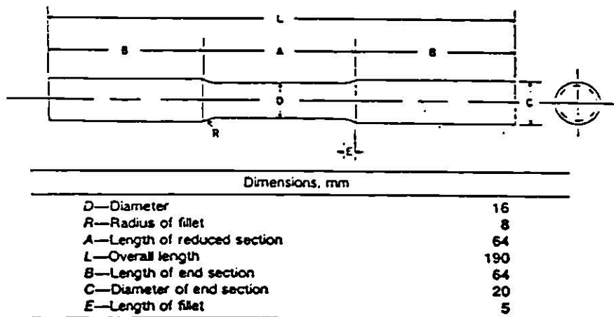
FIG. 17 Standard Tension Test Specimen for Malleable Iron
