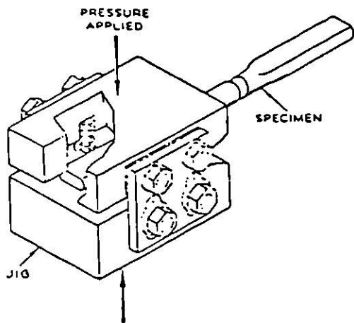
10 Squeezing Jig for Flattening Ends of Full-Size Tension Test Specimens
