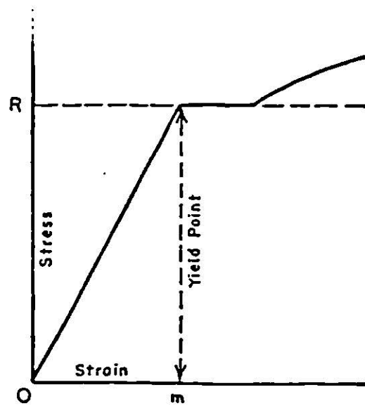
FIG. 23 Stress-Strain Diagram Showing Yield Point Corresponding with Top of Knee
