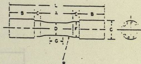
FIG. 13 Tension Test Specimens for Large-Diameter Tubular Products
