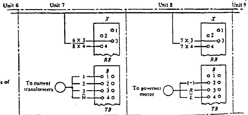
(c) Interconnection diagram
