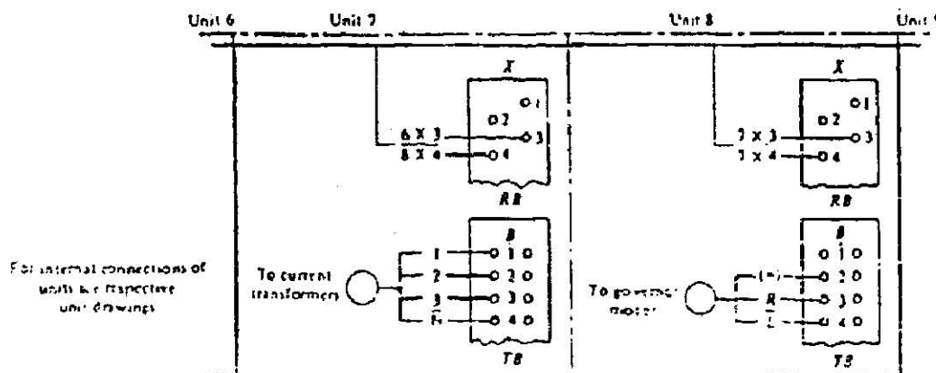
(c) Interconnection diagram
