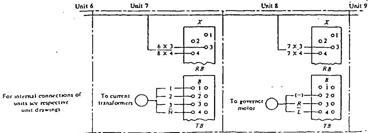
(c) Interconnection diagram
