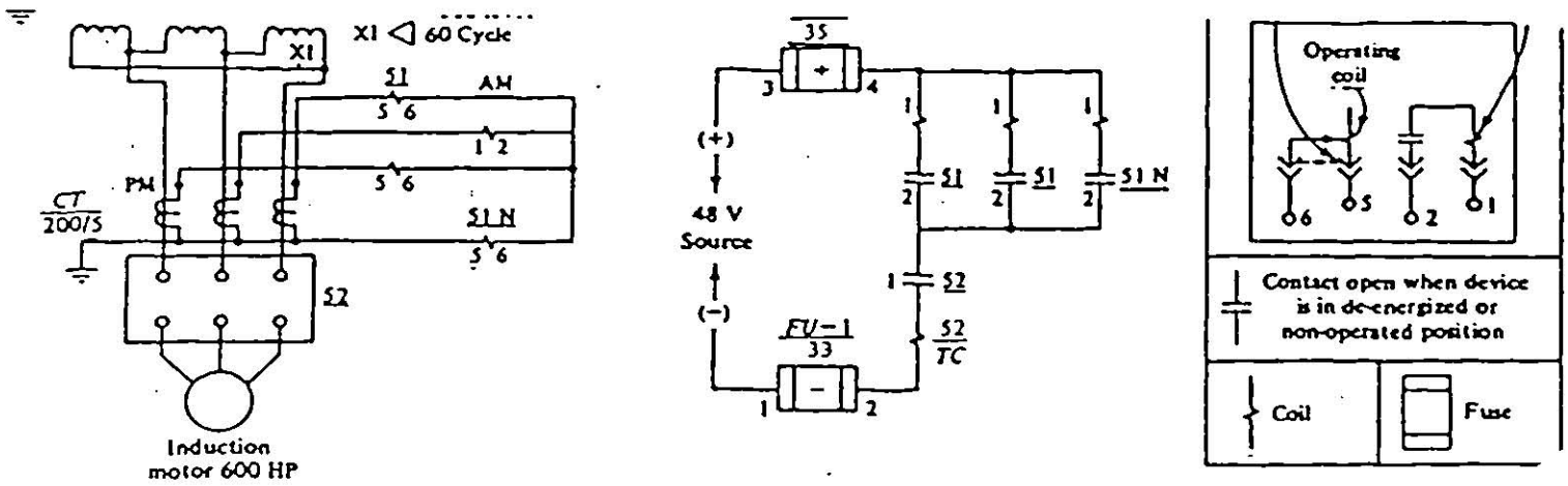
(a) Elementary control diagram
