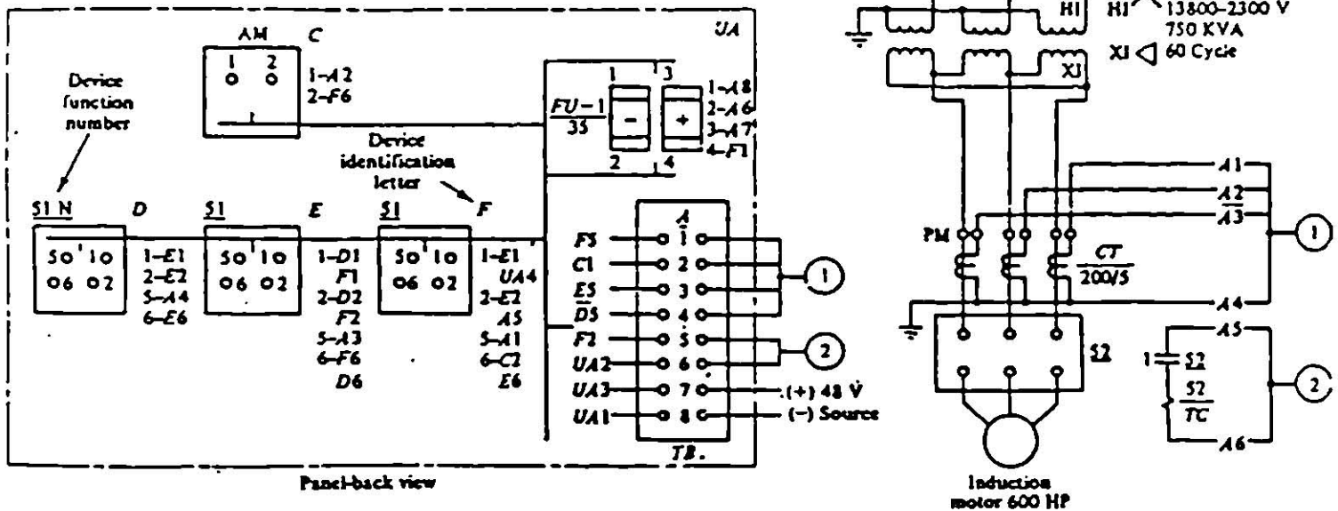
(b) Connection diagram
