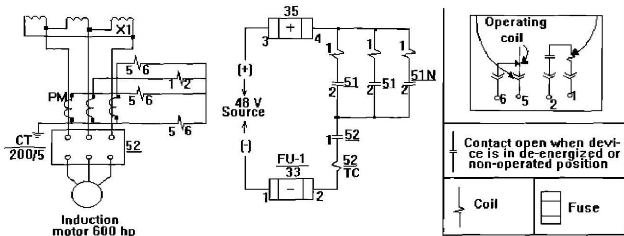
[a] Elementary control diagram
